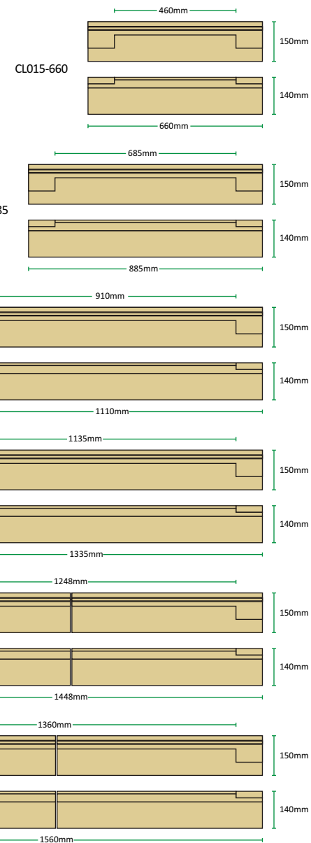
Plan and Elevation of our standard opening sizes
